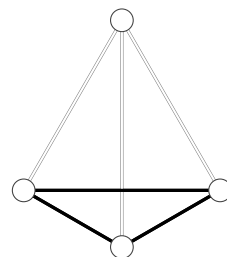
Subcase 2
