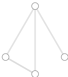
Subcase 1
